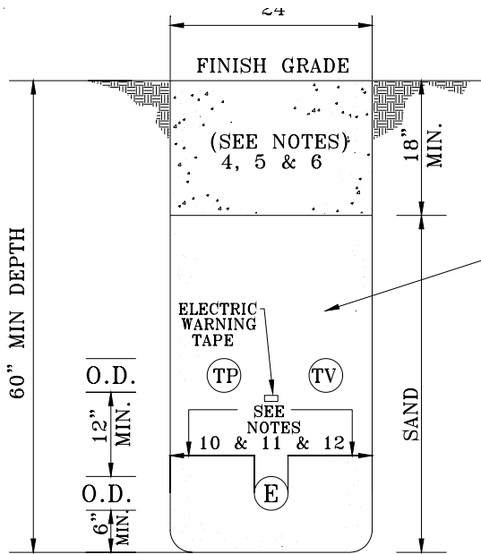
TYPICAL PRIMARY OR SECONDARY TRENCH
