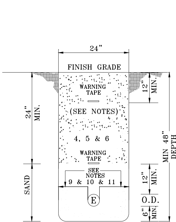
TYPICAL SECONDARY / SERVICE TRENCH ELECTRIC ONLY
