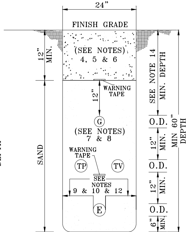
TYPICAL SERVICE TRENCH JOINT TRENCH APPLICATION
