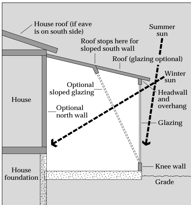
A well-designed overhang may be all that is necessary to shade a vertically sloped interior sunspace wall.
