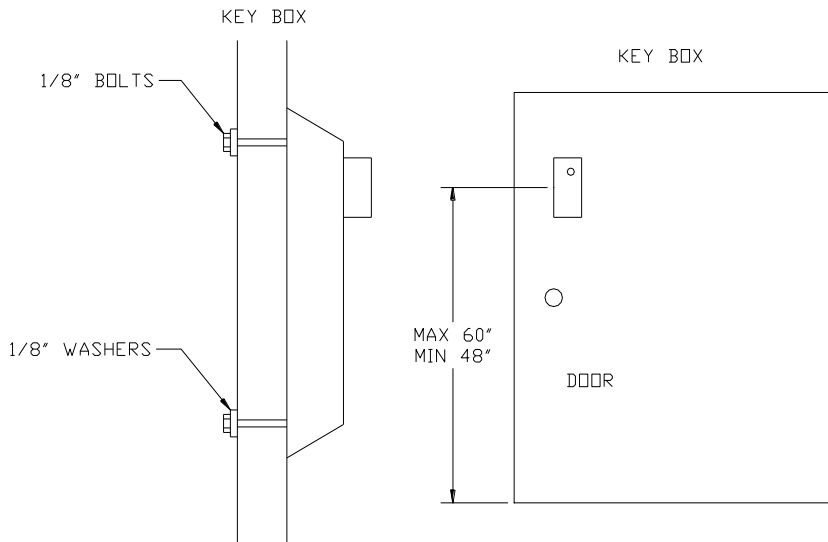
RECOMMENDED INSTALLATION DETAIL
