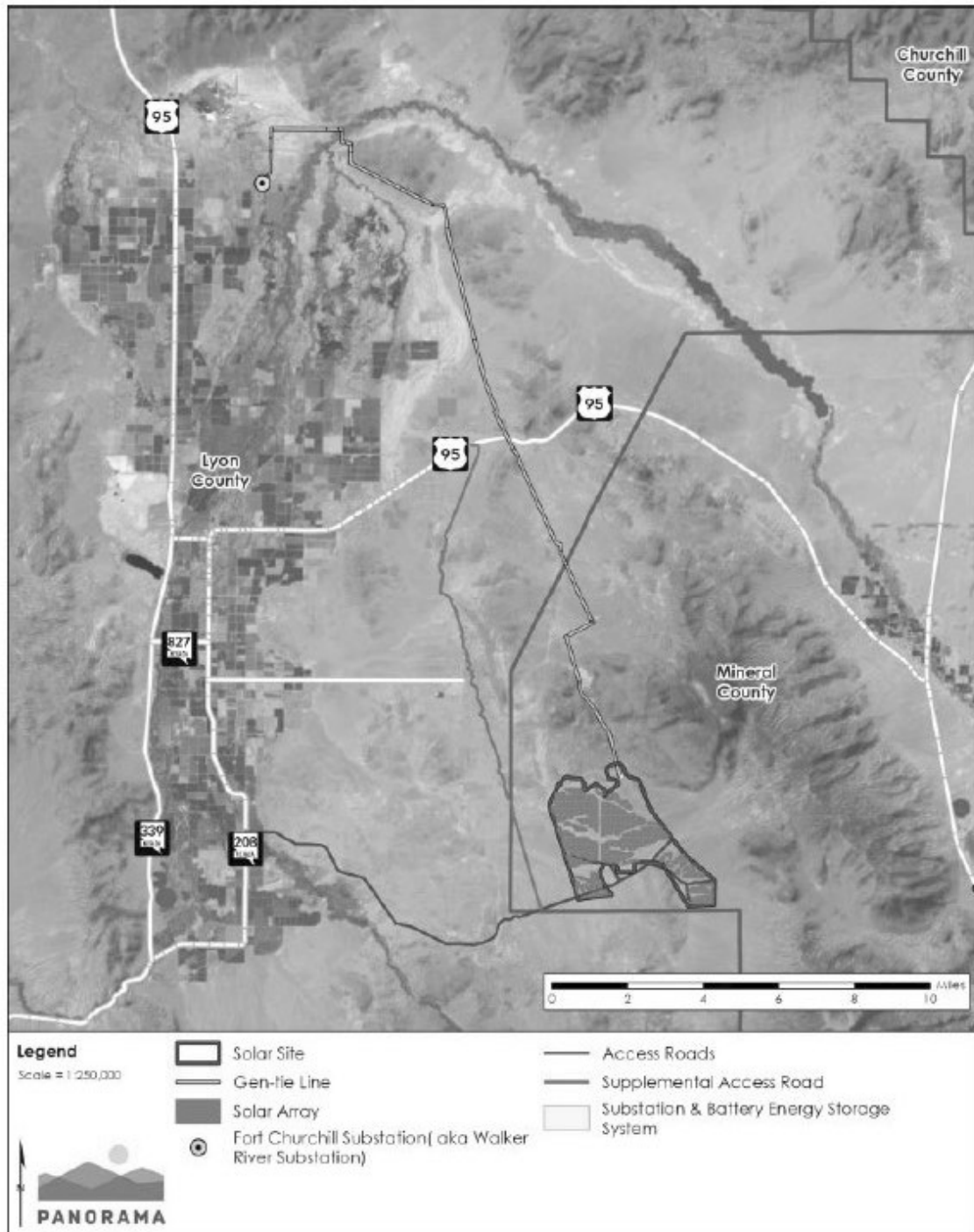
Figure 3-2 Project Components
