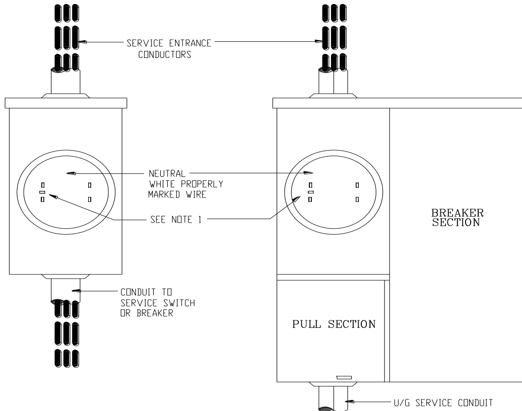
INDIVIDUAL METER SOCKET SEE NOTE 2
