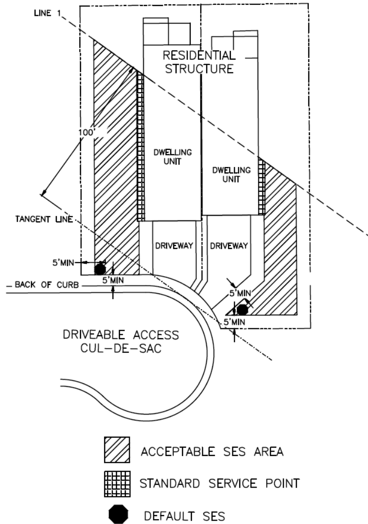
Figure 4. Flag Lot in a Cul-de-Sac
