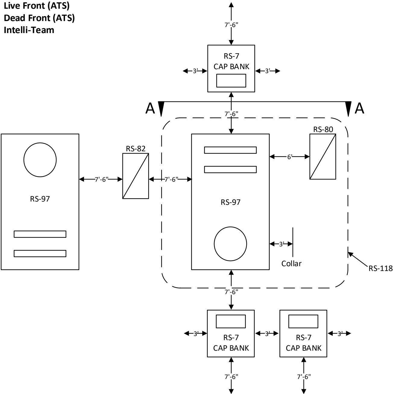
Plan View
