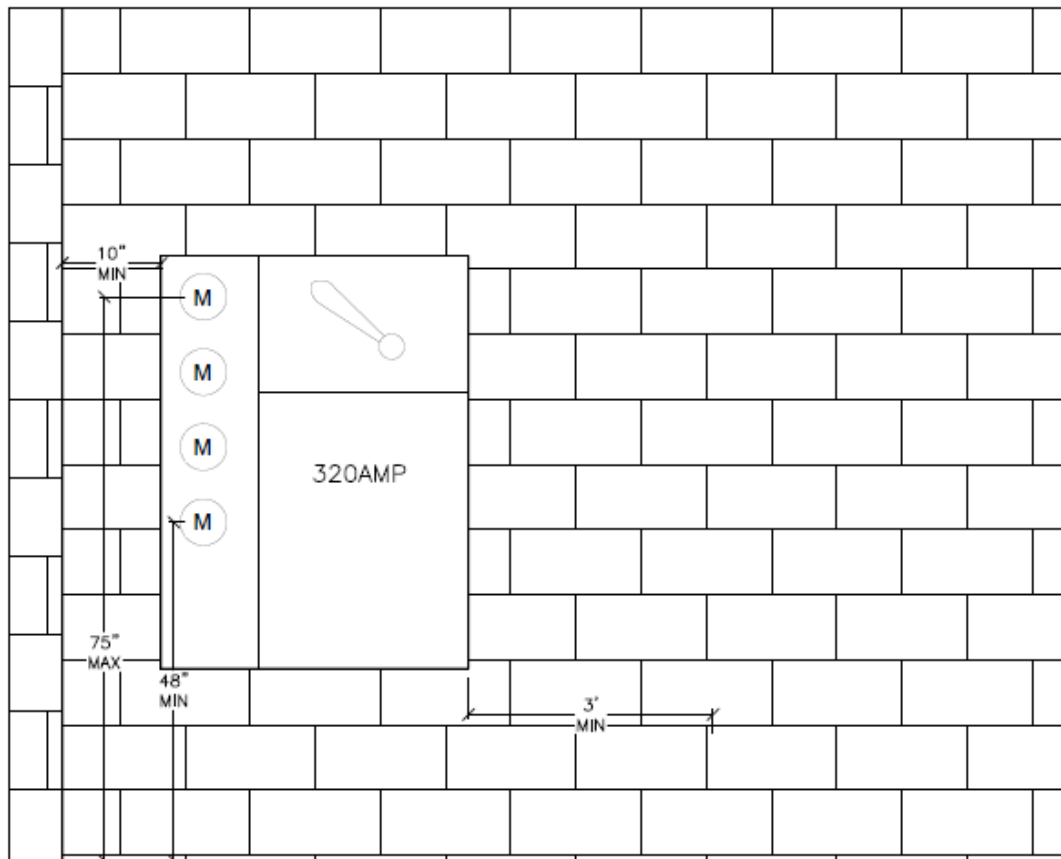
Figure 8. Free-standing Meter Wall
