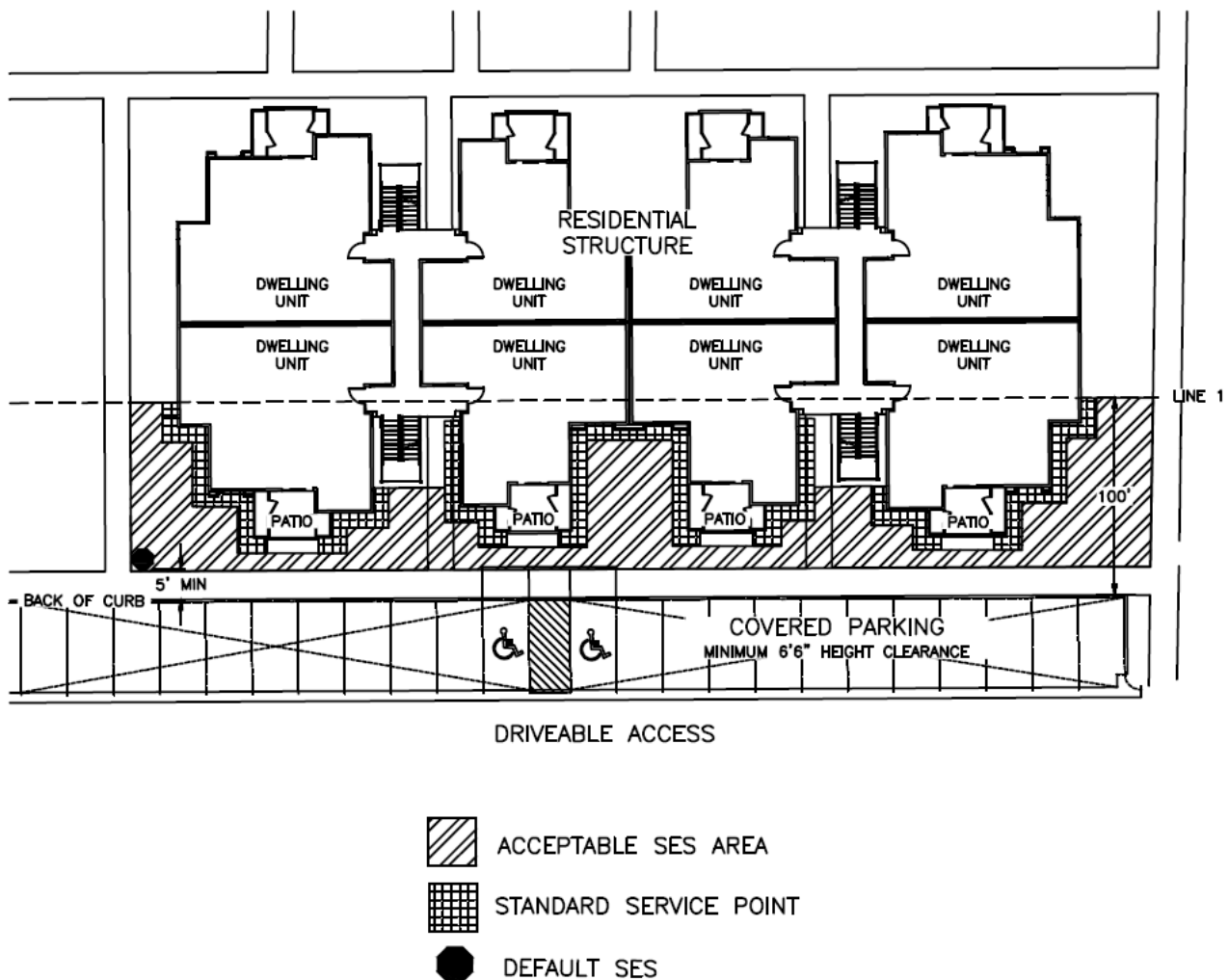
Figure 1. Locating the Standard Service Point
