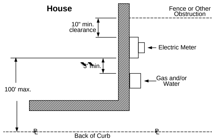
Figure 6. Clearances Around the Meter
