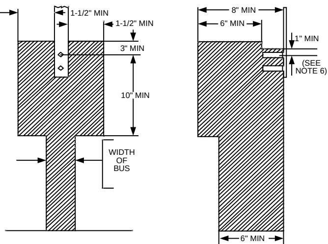
FIGURE 4 REQUIRED UNOBSTRUCTED WORKING SPACE FOR ALL TERMINATIONS
