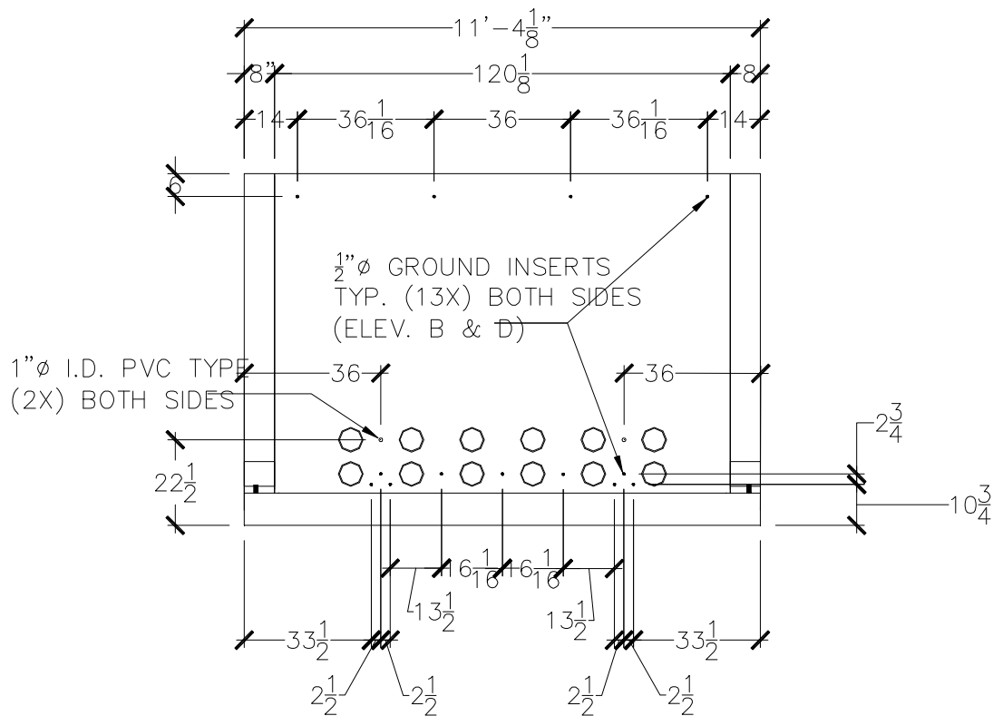
\frac{1}{2}" GROUND INSERTS LOCATION
