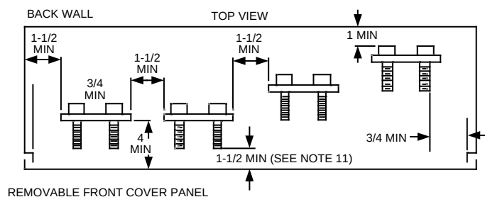
FIGURE 2 SPACING REQUIREMENTS FO TERMINATING FACILITIES (SIDE BY SIDE OR STAGGERED)
