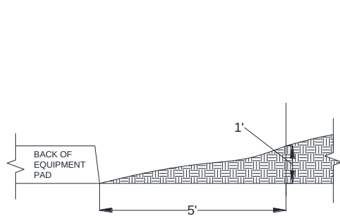
Figure 1 Maximum Allowable Grade Change
