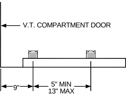
SIDE VIEW OF VT MOUNTING
