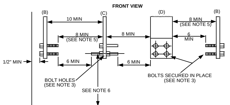
FIGURE 3 SPACING REQUIREMENTS FOR TERMINATING FACILITIES ACCESSIBLE FROM (A) FRONT ONLY, (B) ONE SIDE ONLY, OR (C) FROM EITHER SIDE (SEE NOTES 3 & 4)
