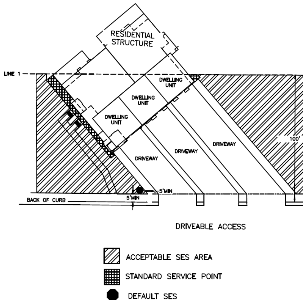
Figure 3. Front of House that is Not Parallel to the Back of Curb
