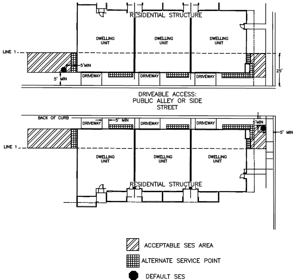
Figure 2. Locating an Alternate Service Point
