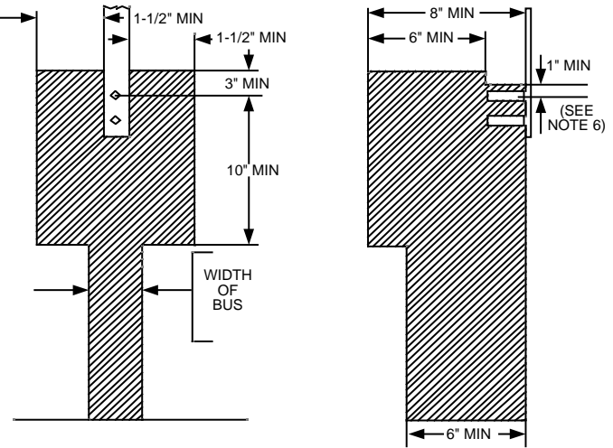
FIGURE 4 REQUIRED UNOBSTRUCTED WORKING SPACE FOR ALL TERMINATIONS
