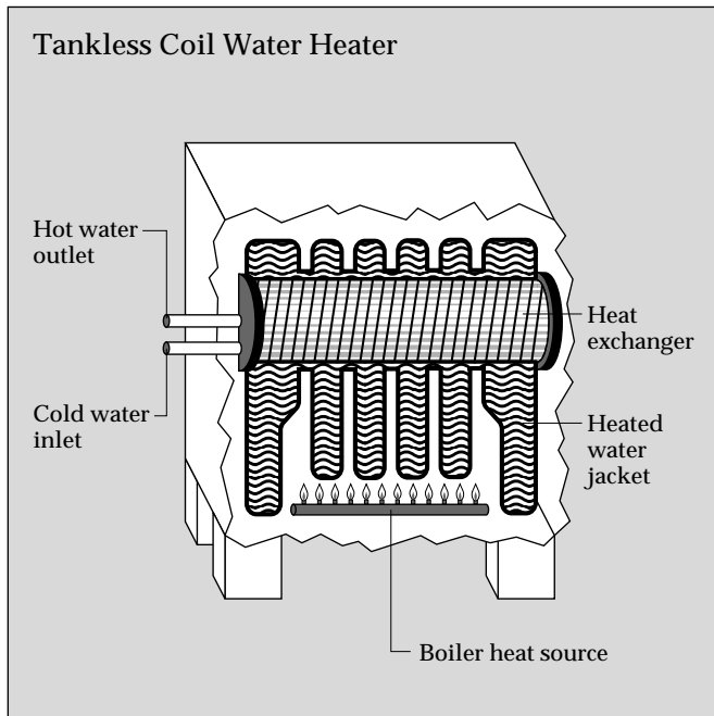
A tankless coil water heater uses a heat exchanger in the boiler to heat water.
