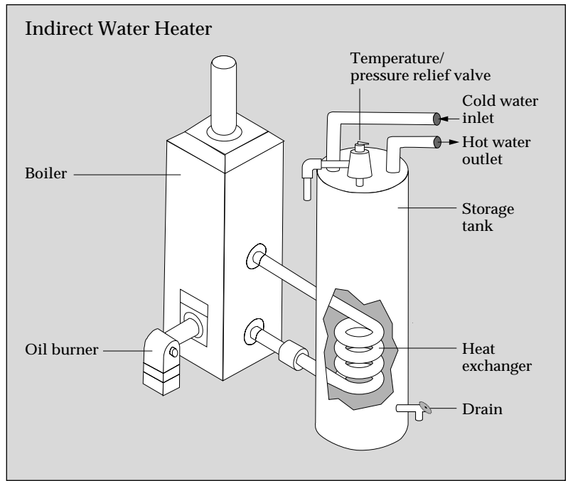
A combination of an indirect water heater and a highly efficient boiler can provide a very inexpensive method of water heating.
